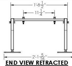
END VIEW RETRACTED
