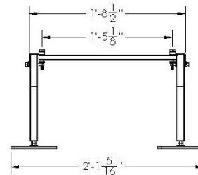
END VIEW EXPANDED
